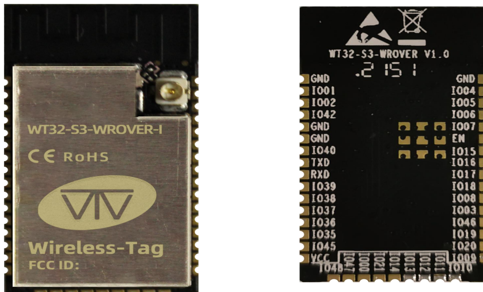
Figure 2 Pin Layout
