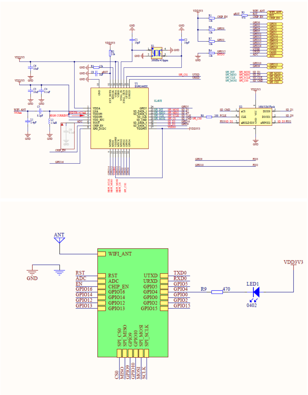
Figure -7 WT8266-S2 Schematics
