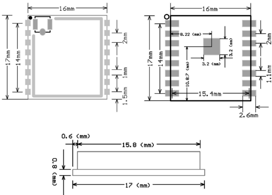
Figure -4 Module Size
