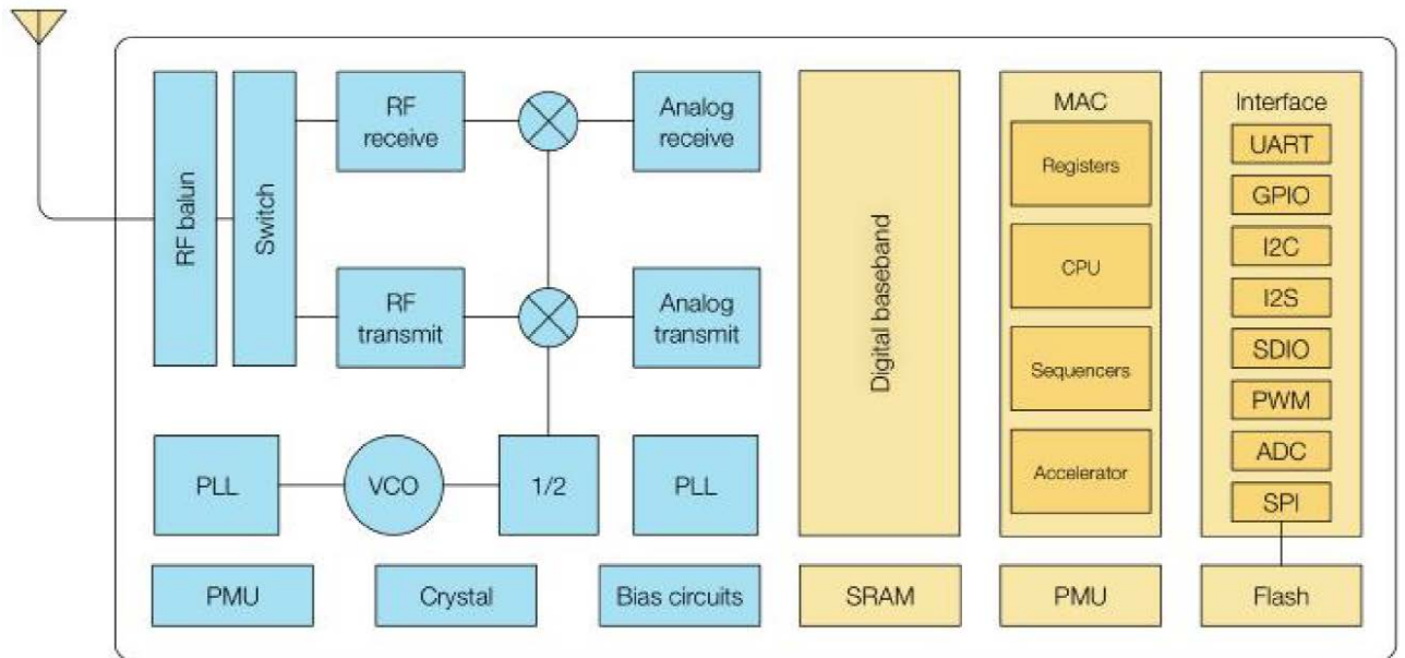
Figure-1 System Diagram
