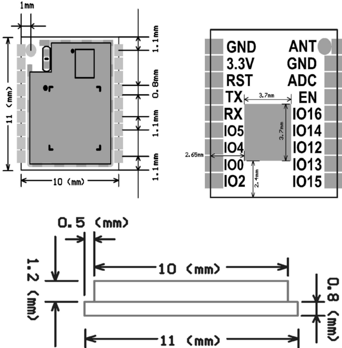
Figure -4 Module Size
